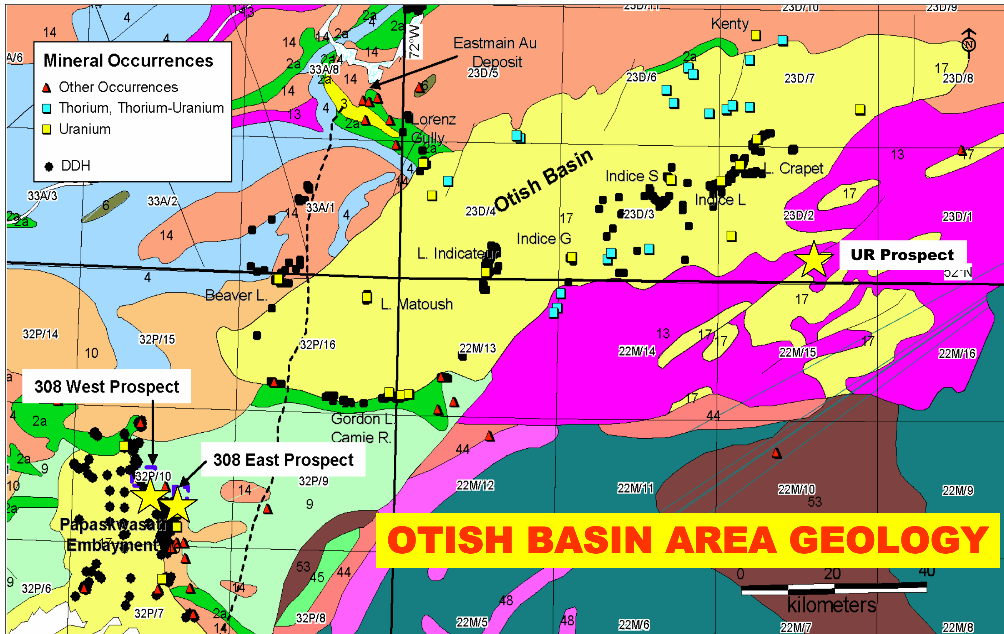
Figure 4a: Regional Geology, Otish Basin and Papaskwasati Embayment (from MRNFQ, 2005).
